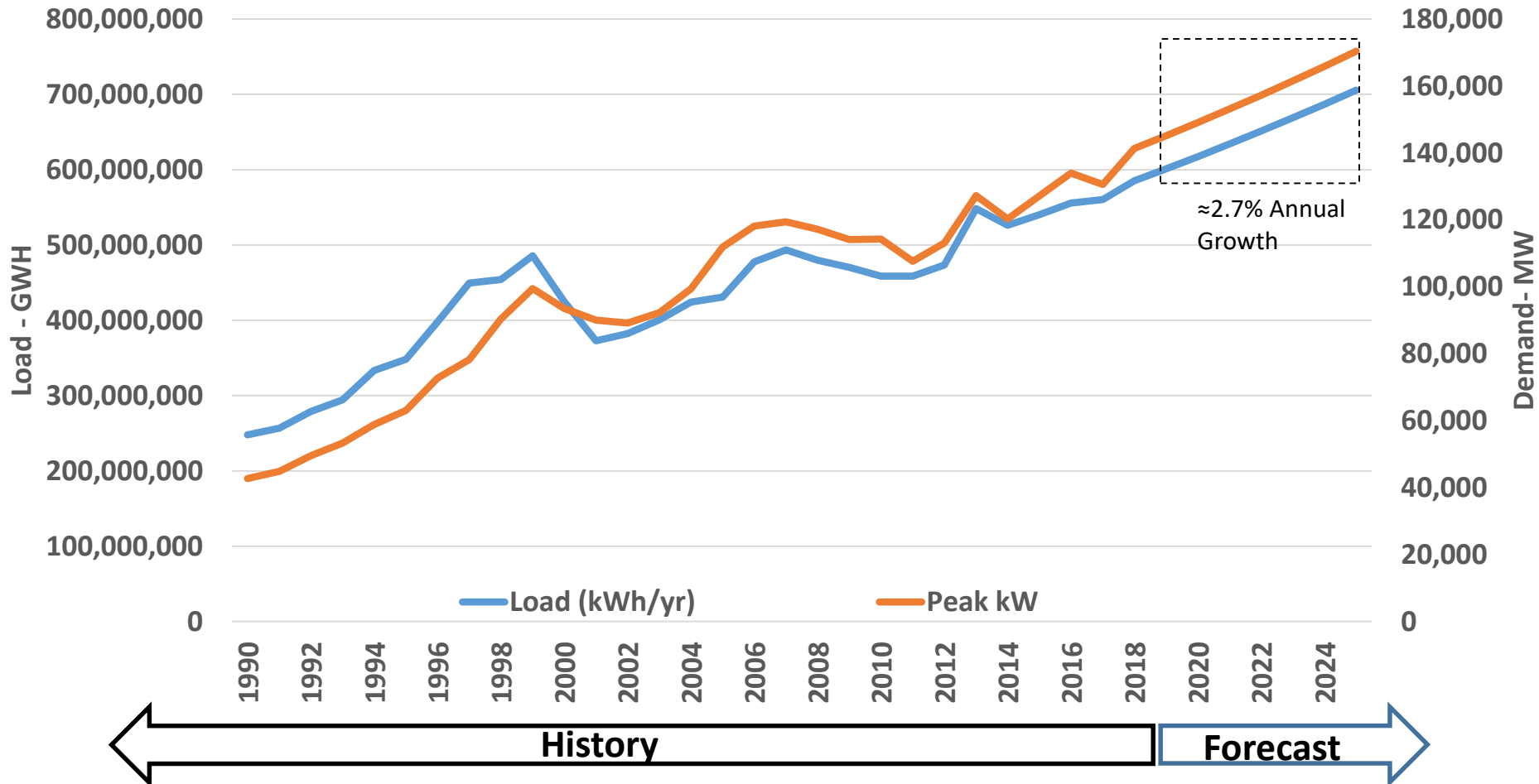
VEA Load History/Forecast
